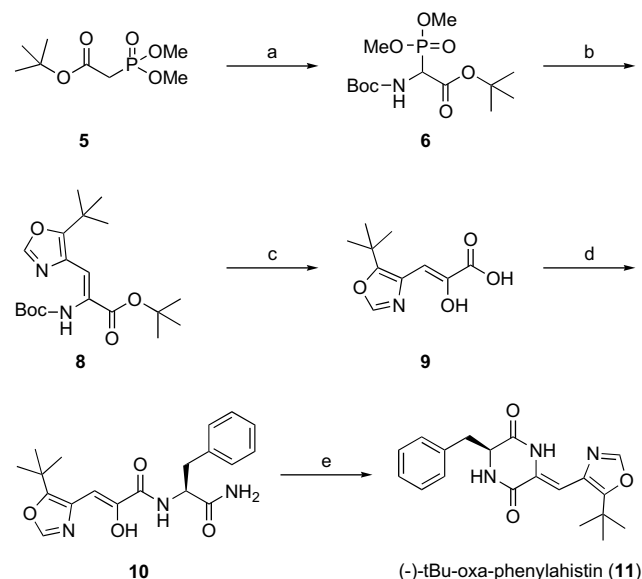
Scheme 2. Synthesis of a phenylahistin derivative 11 ((-)- tert -butyl-oxa-phenylahistin) via acid catalyzed monodehydroDKP synthesis. Reagents and conditions; (a) (i) NaH, TsN_3 , rt, 2 h; (ii) Boc-NH 2 , cat. Rh_2(OAc)_4 , toluene, reflux, 1 h, 51% in two steps; (b) 5- tert -butyl-4-oxazolecaboxaldehyde 7 , Cs_2CO_3 , DMF, rt, 14 h, 47%; (c) 4 M HCl/dioxane, rt, 1 h, 76%; (d) HCl·H-Phe-NH 2 , EDC·HCl, HOBT·H 2 O, Et 3 N, DMF, rt, 14 h, 43%; (e) 5 mol % p -TsOH, toluene, reflux, 6 h, 20%.
