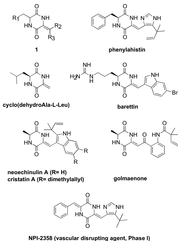
Figure 1. Chemical structures of naturally occurring monodehydroDKPs and DKP anticancer agent NPI-2358.
