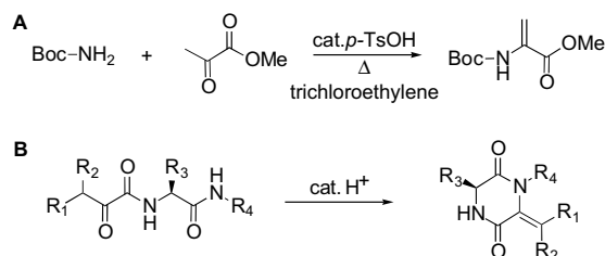
Scheme 1. (A) Gladiali's method for the synthesis of dehydroamino acid derivatives. (B) A new synthetic strategy of monodehydroDKP based on A.
