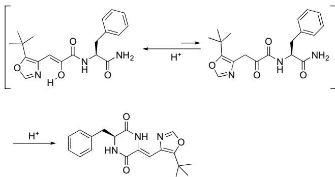
Scheme 3. Keto-enol tautomerism of \beta -aryl- \alpha -keto acid derivative.
