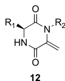
Figure 2. MonodehydroDKP synthon with an exo -olefin structure.
